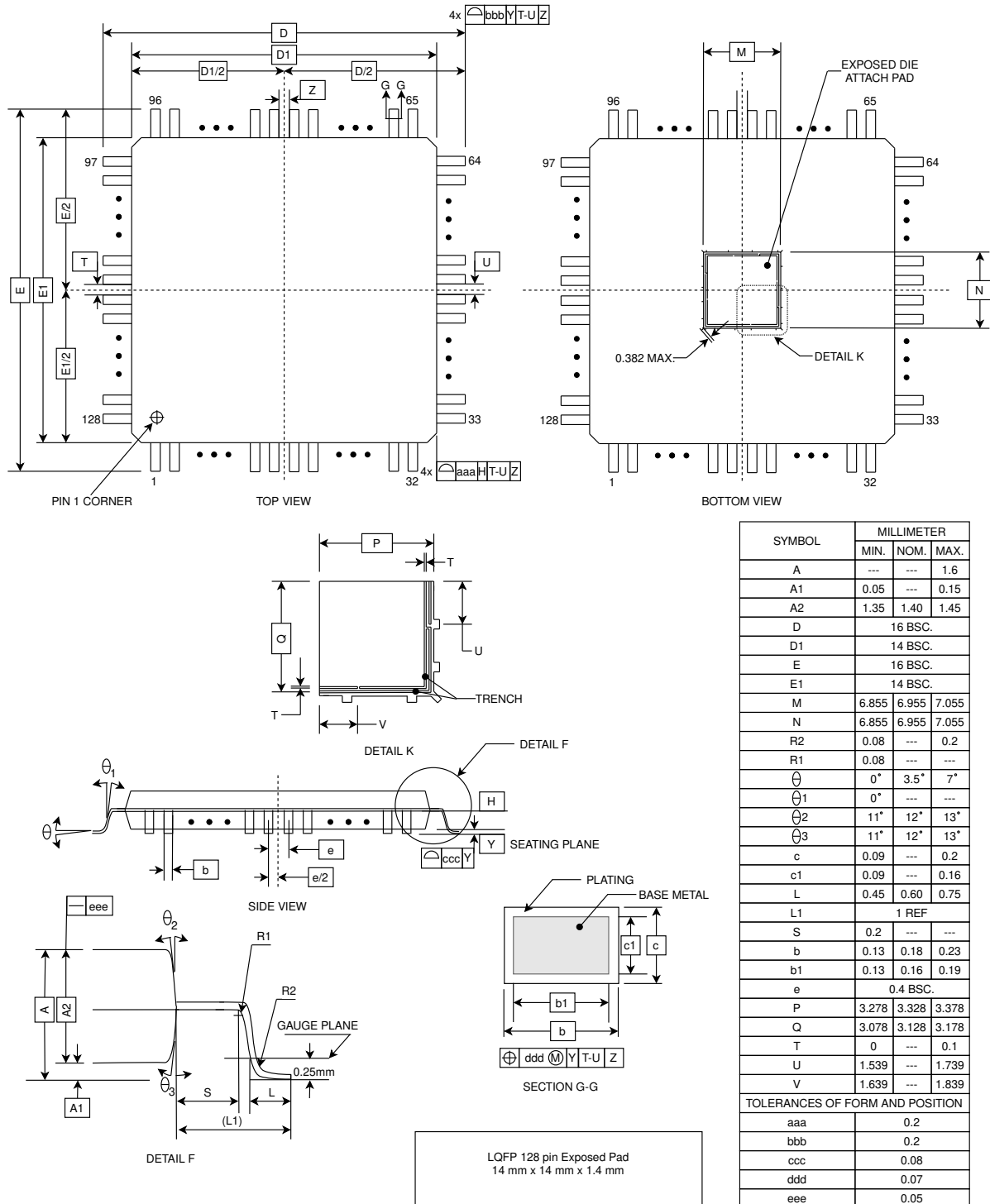
Figure A.1.1-1: Package Drawing
